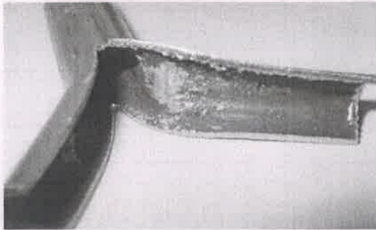
Pitting corrosion observed on cut cross section of a cupro-nickel tube from a turbine lub-oil cooler
