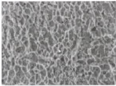
Ductile fracture
