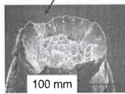
Fracture surface of steel wire loaded in tension. Courtesy of F. Roering, CC Technologies, Dublin, OH. Used with permission.
