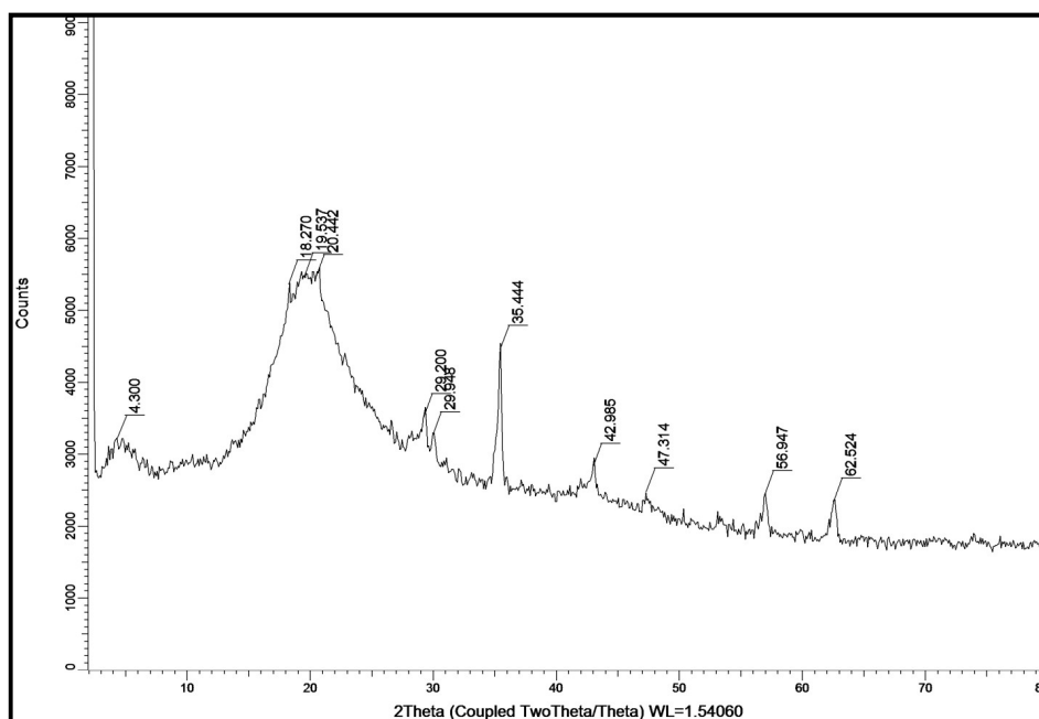
Fig.5.2: X-ray diffractogram of iron oxide nanoparticles.
